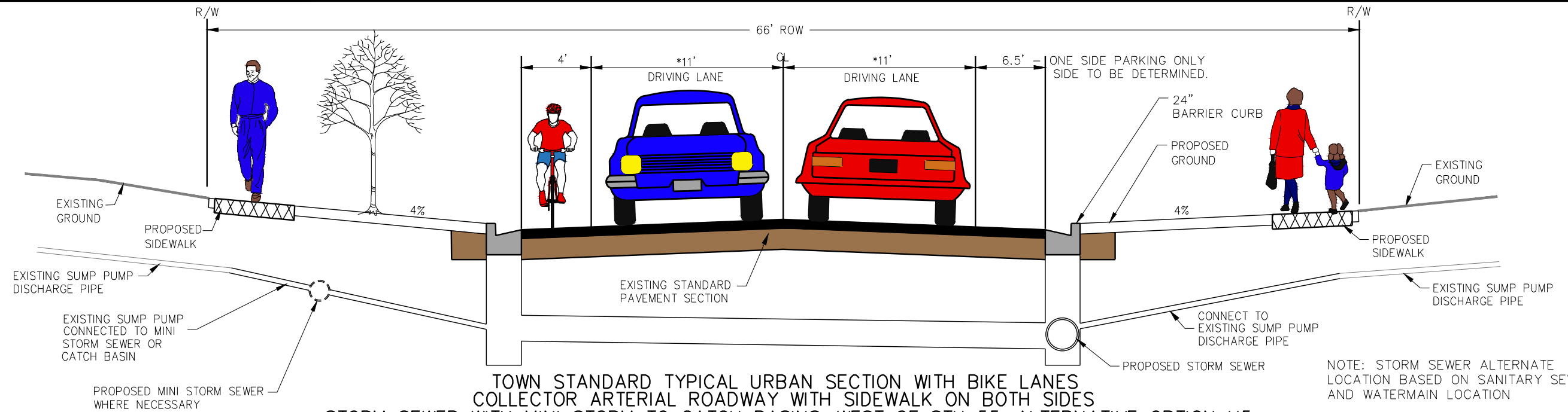
TOWN STANDARD TYPICAL URBAN SECTION PLAN VIEW NO SCALE
