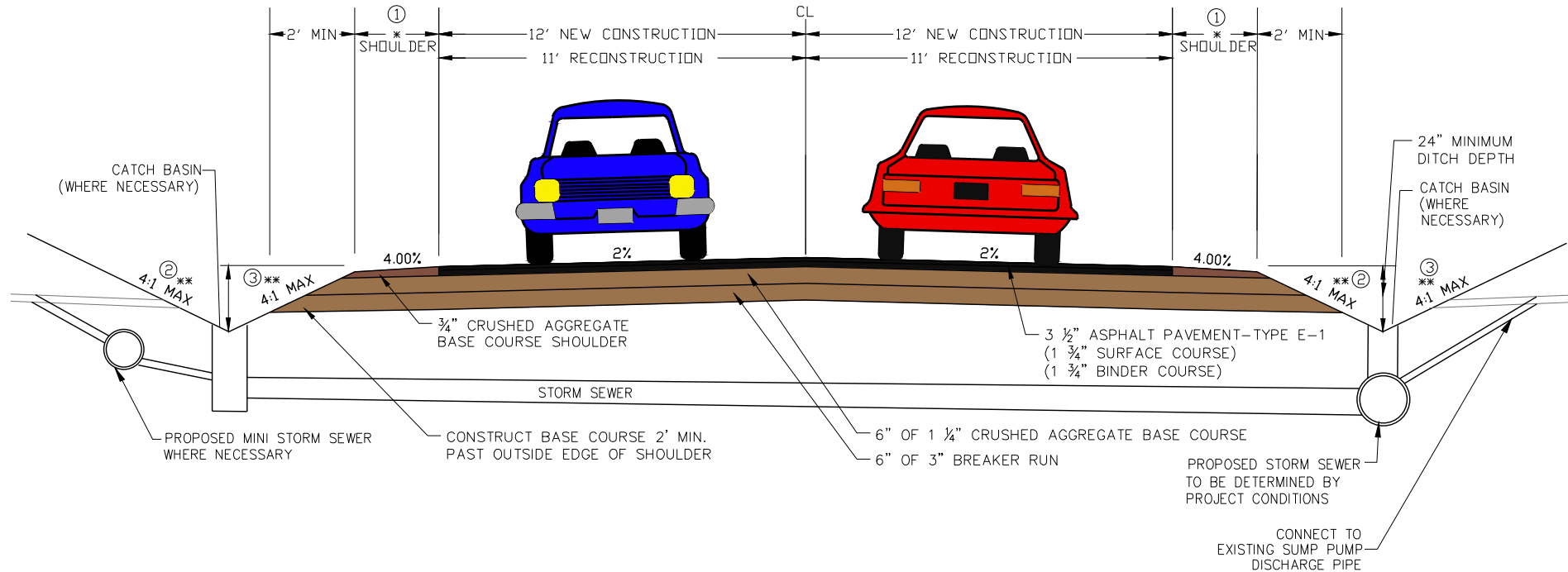
TYPICAL SECTION – RESIDENTIAL STREET STORM SEWER IN DITCH – ALTERNATIVE OPTION R3 EAST OF STH 55
